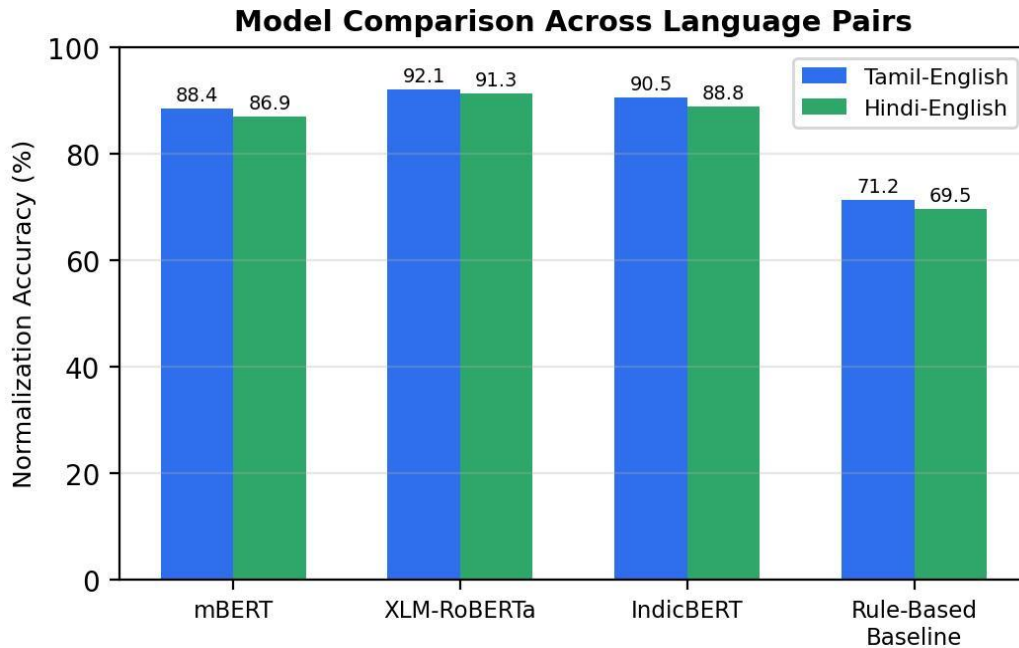
Fig. A.3. Model Comparison Across Language Pairs
